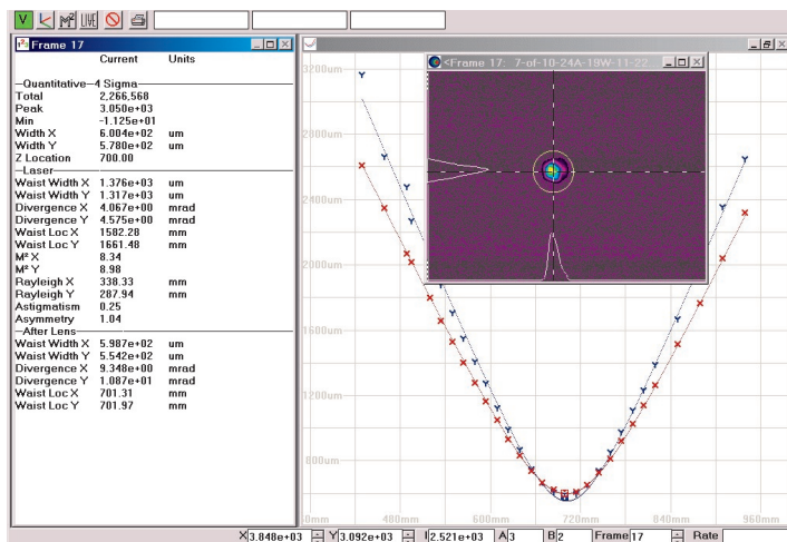
Lucia-30-M Output Beam Quality Measurement
